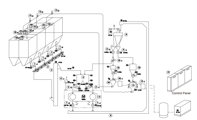
Milling and Separating System Flow
